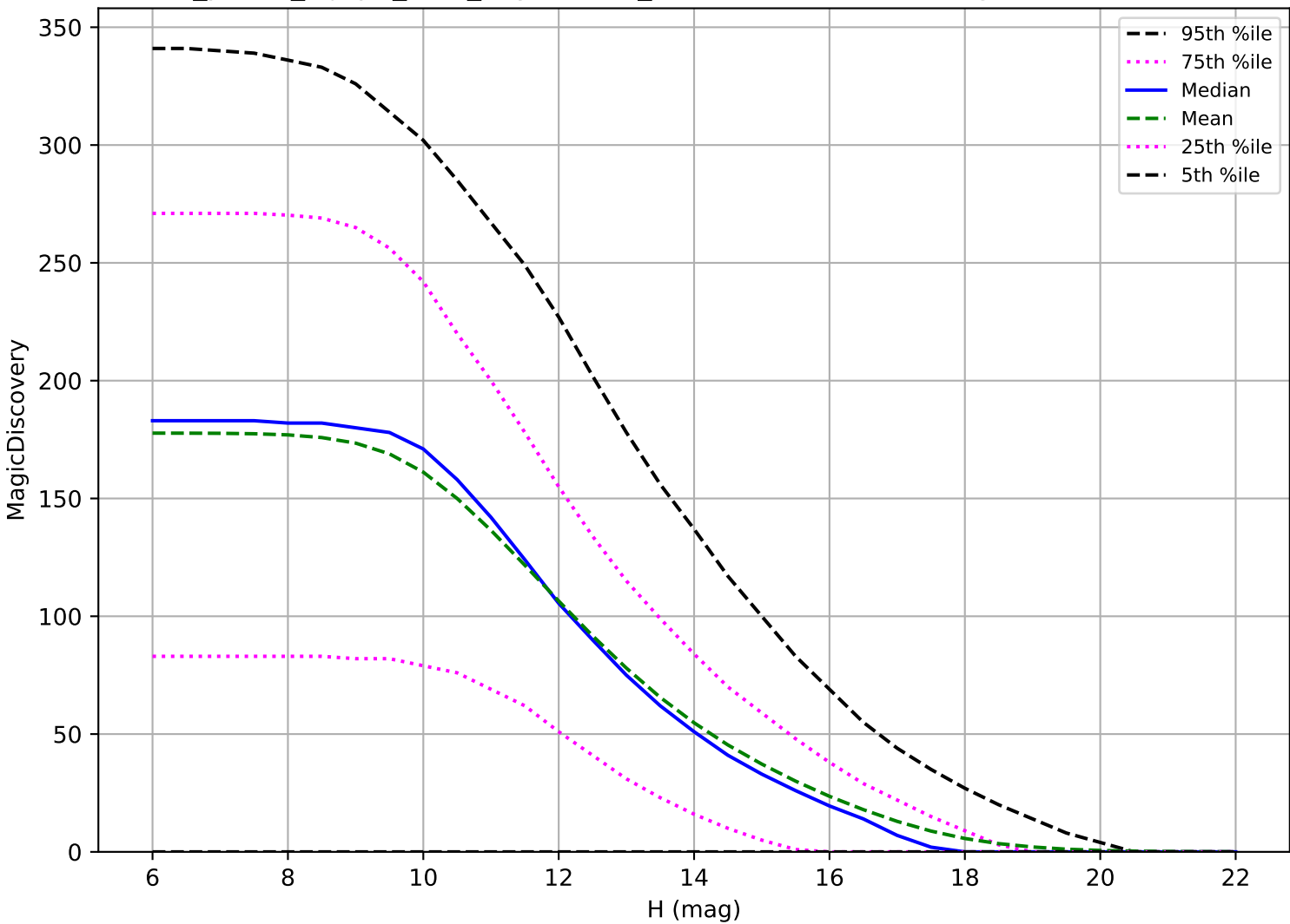
roll_pause_mjdp0_v3.4_10yrs: OCC_r5 6 detections in 60 nights detection loss
