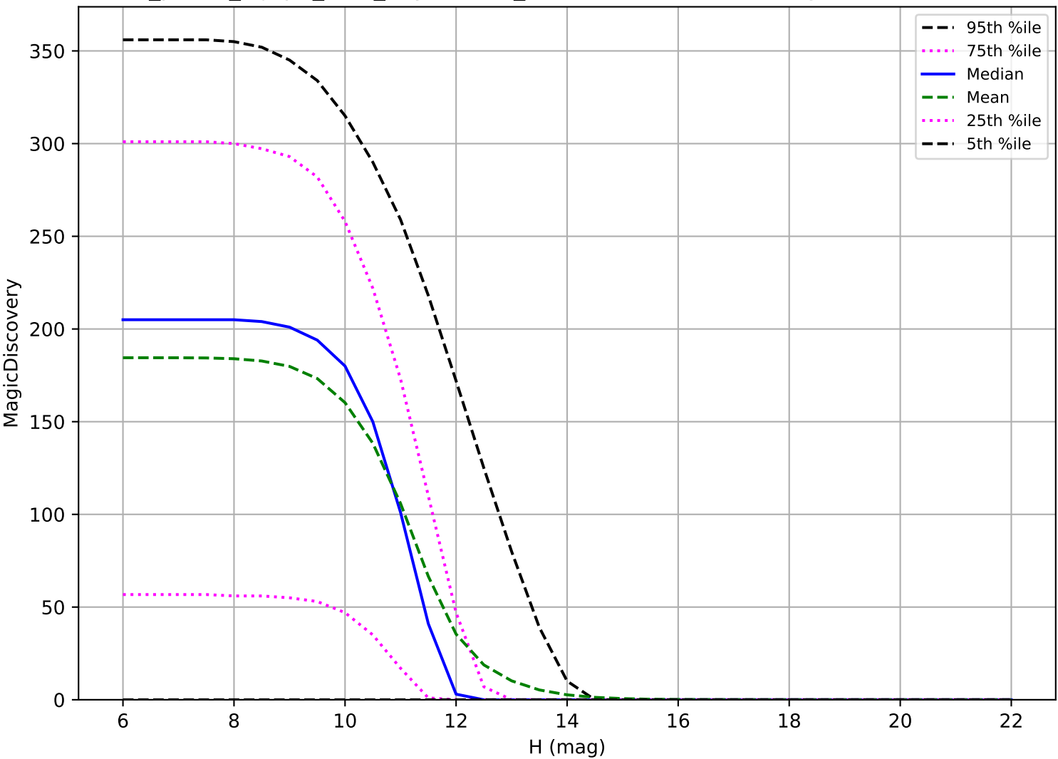
roll_pause_mjdp0_v3.4_10yrs: OCC_r20 6 detections in 60 nights detection loss
