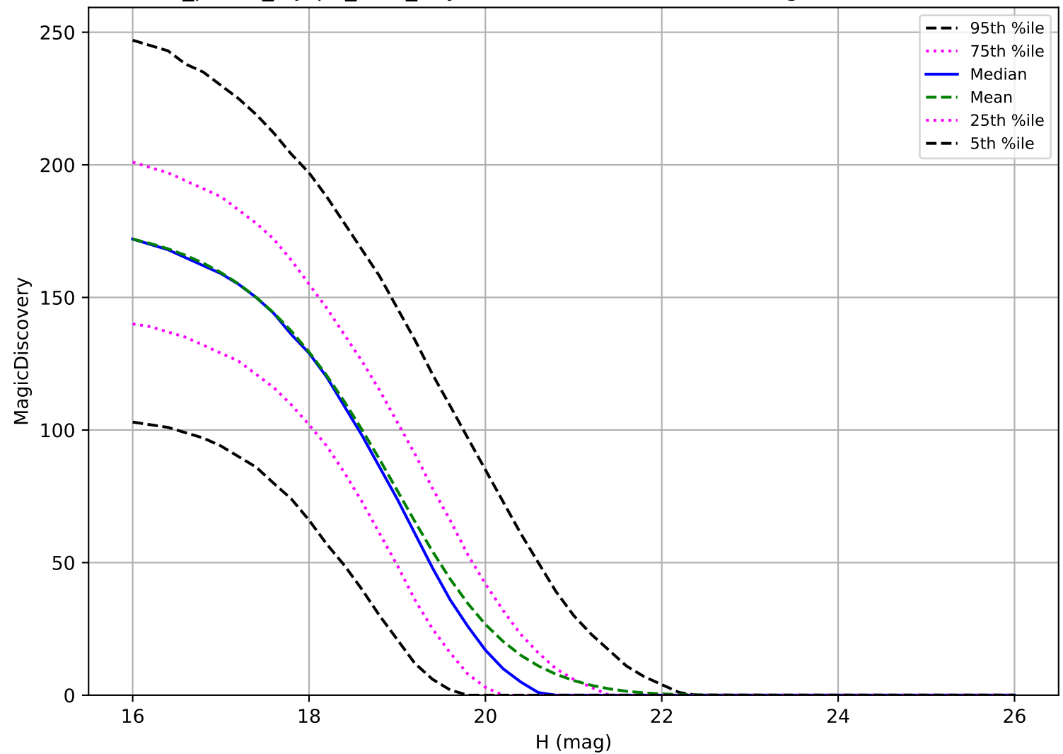
roll_pause_mjdp0_v3.4_10yrs: MBA 6 detections in 60 nights detection loss
