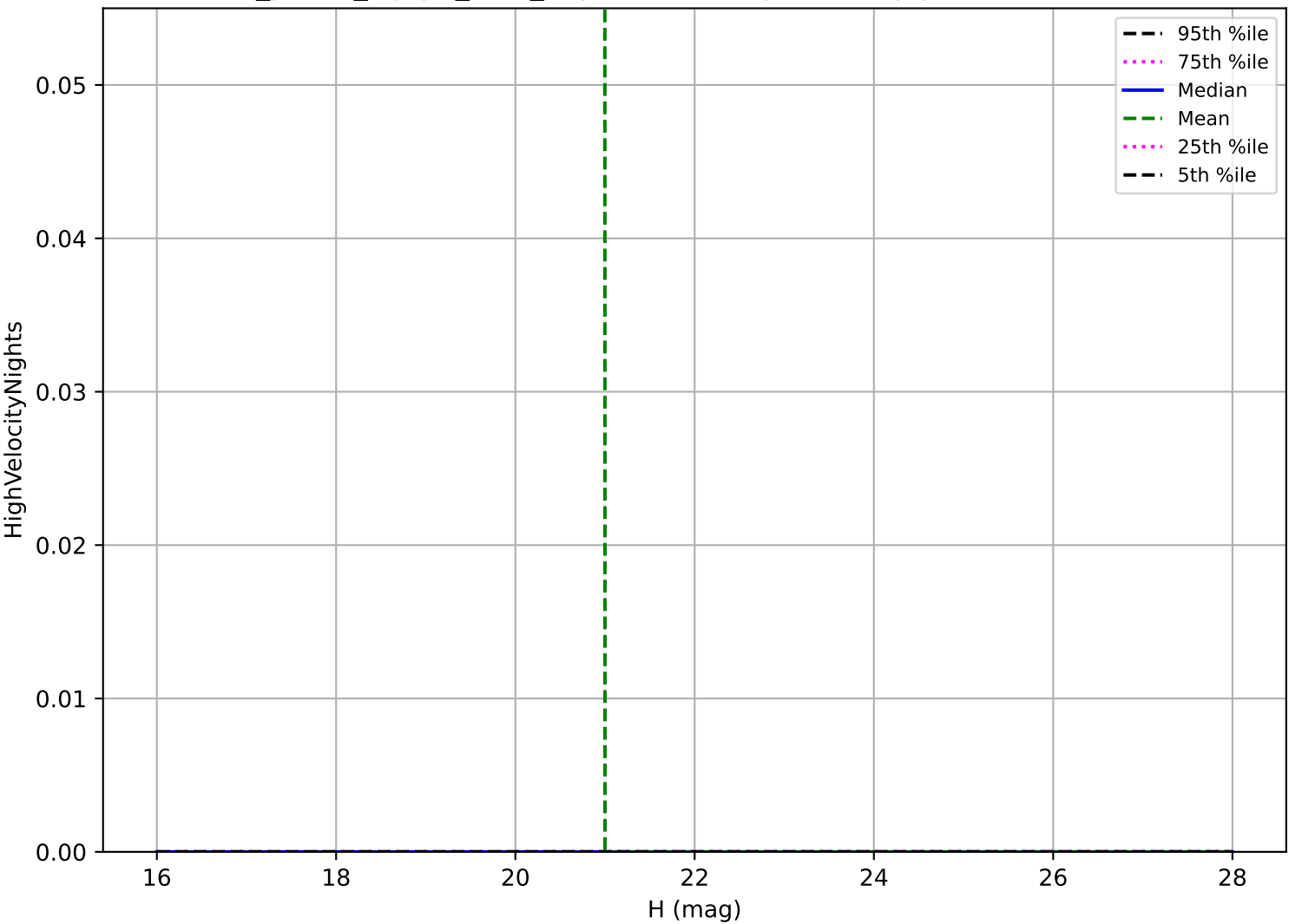
roll_pause_mjdp0_v3.4_10yrs: Vatira High velocity pair detection loss
