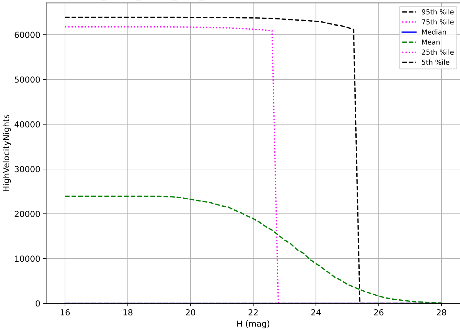
roll_pause_mjdp0_v3.4_10yrs: PHA High velocity pair detection loss
