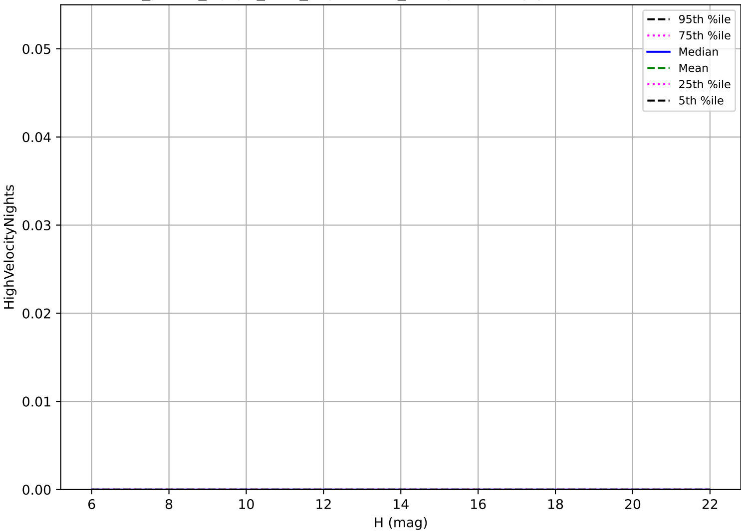
roll_pause_mjdp0_v3.4_10yrs: OCC_r5 High velocity pair detection loss
