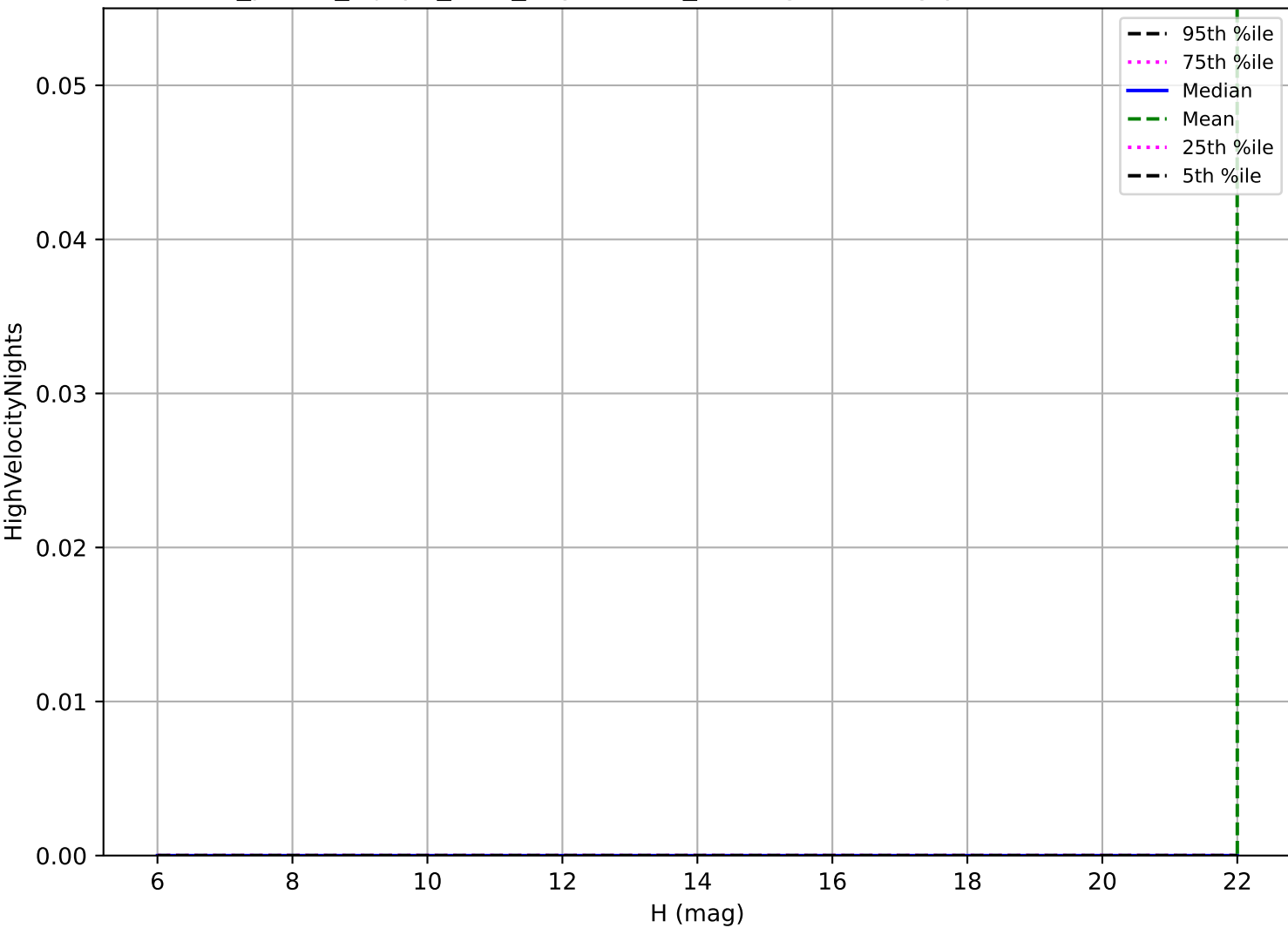
roll_pause_mjdp0_v3.4_10yrs: OCC_r20 High velocity pair detection loss
