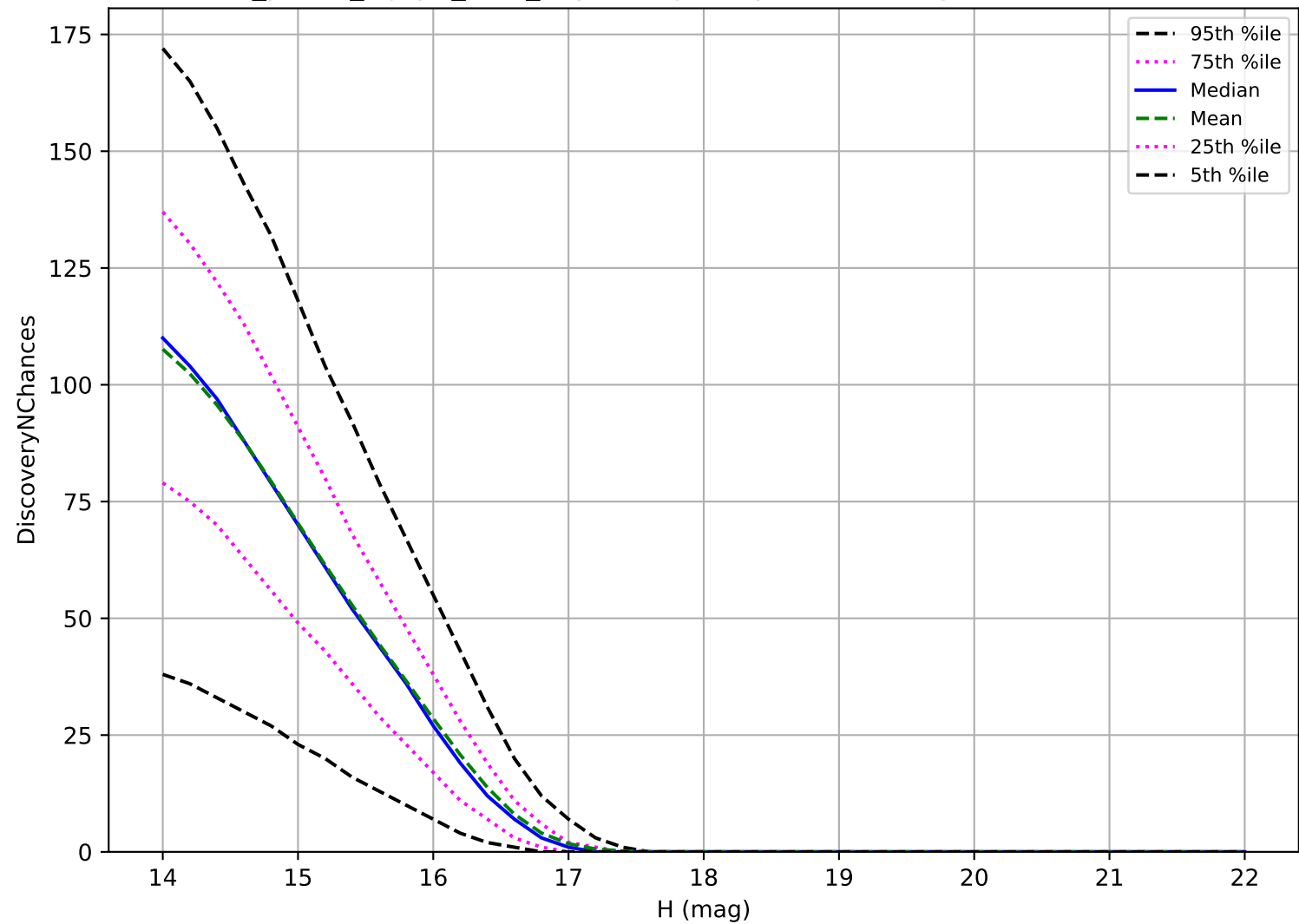
roll_pause_mjdp0_v3.4_10yrs: Trojan 3 pairs in 15 nights detection loss
