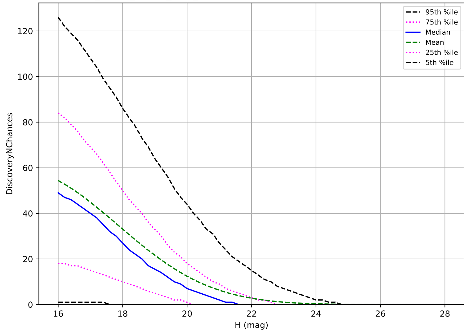
roll_pause_mjdp0_v3.4_10yrs: PHA 3 pairs in 15 nights detection loss
