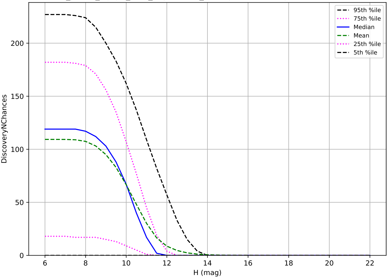
roll_pause_mjdp0_v3.4_10yrs: OCC_r20 3 pairs in 15 nights detection loss
