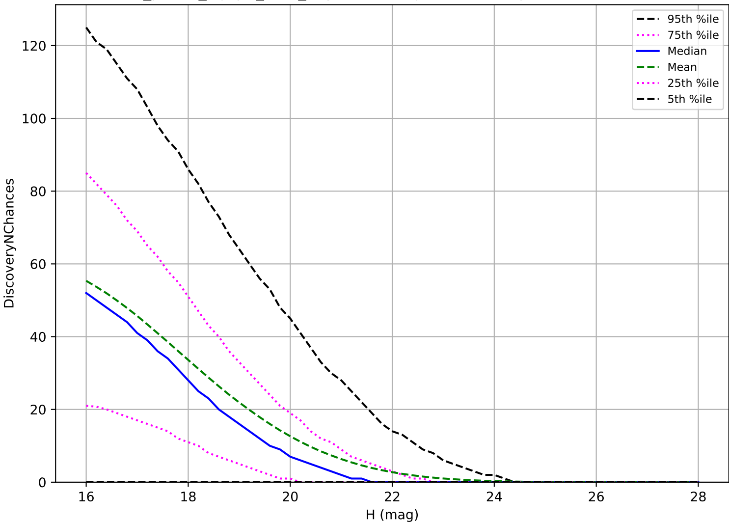
roll_pause_mjdp0_v3.4_10yrs: NEO 3 pairs in 15 nights detection loss
