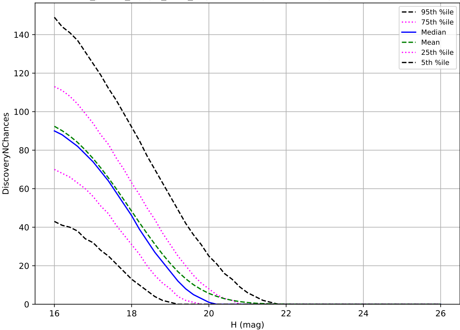
roll_pause_mjdp0_v3.4_10yrs: MBA 3 pairs in 15 nights detection loss
