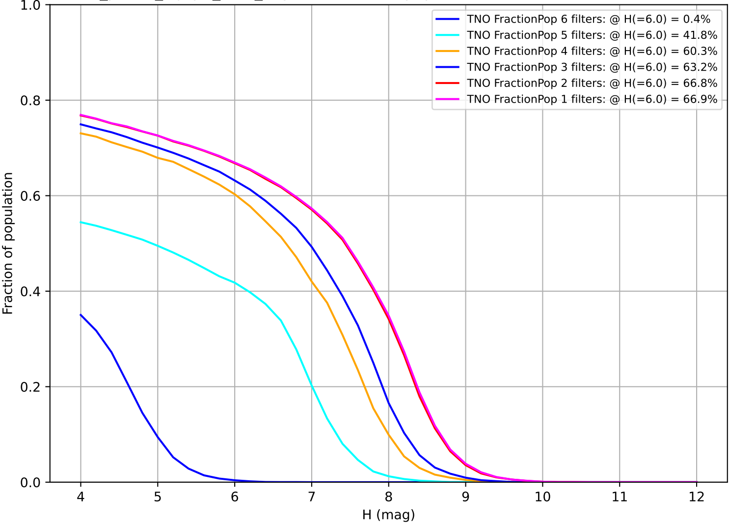
roll_pause_mjdp0_v3.4_10yrs: Fraction of population with colors in X filters TNO
