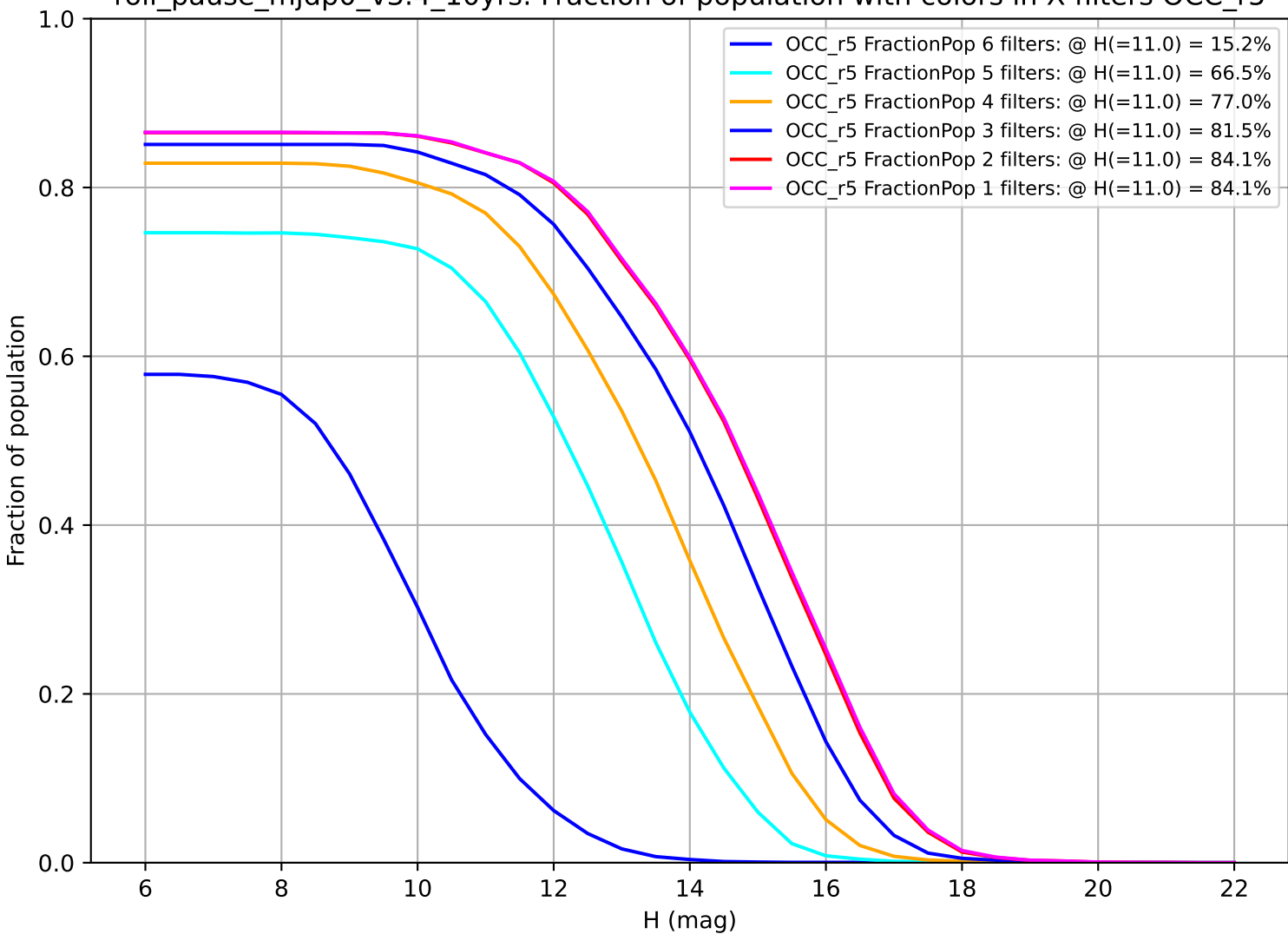
roll_pause_mjdp0_v3.4_10yrs: Fraction of population with colors in X filters OCC_r5
