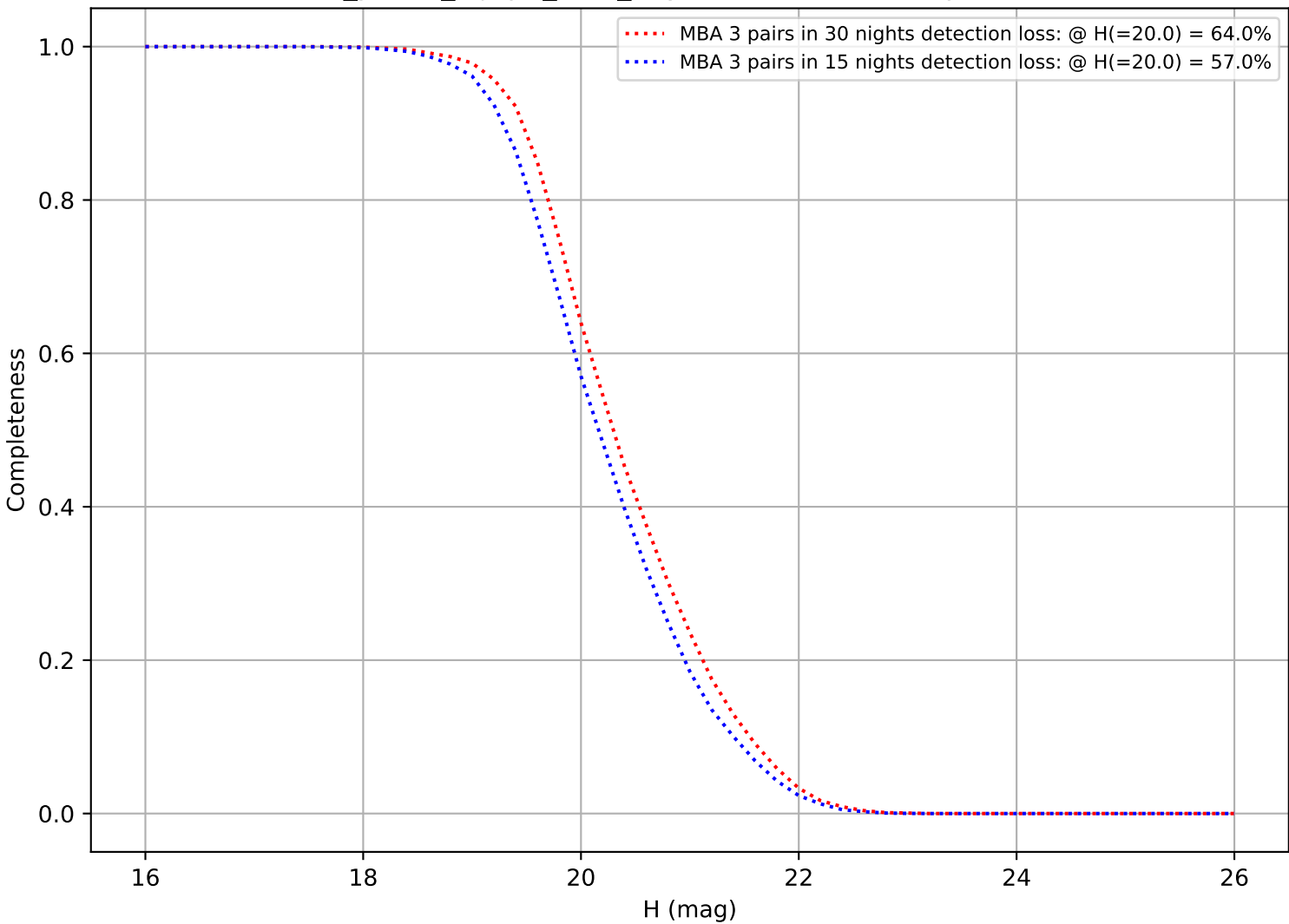
roll_pause_mjdp0_v3.4_10yrs: DifferentialCompleteness
