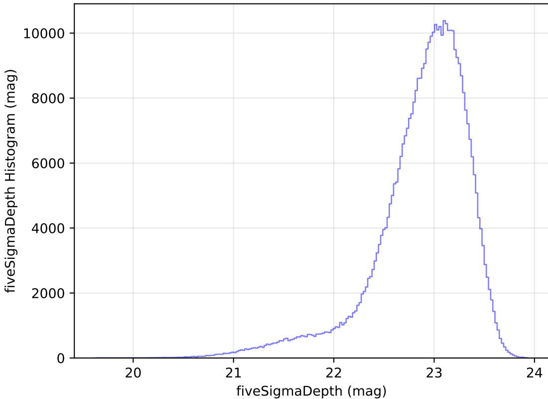
roll_pause_mjdp0_v3.4_10yrs z: fiveSigmaDepth Histogram
