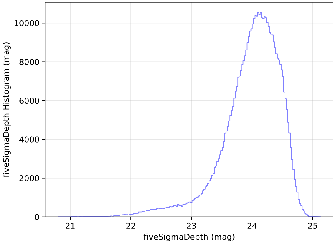
roll_pause_mjdp0_v3.4_10yrs r: fiveSigmaDepth Histogram
