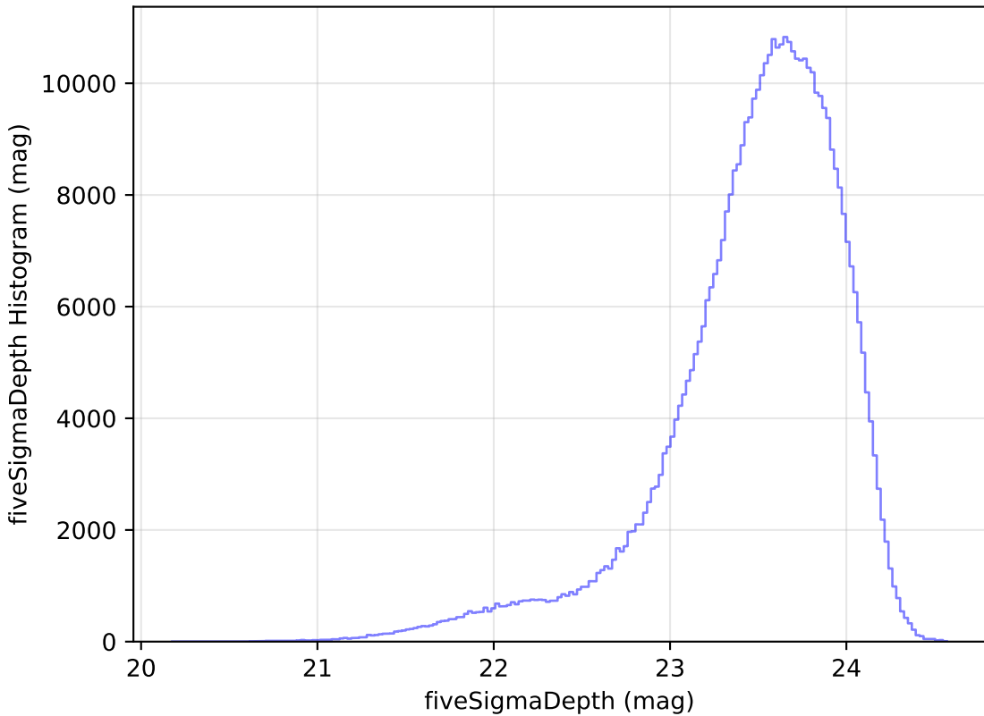
roll_pause_mjdp0_v3.4_10yrs i: fiveSigmaDepth Histogram
