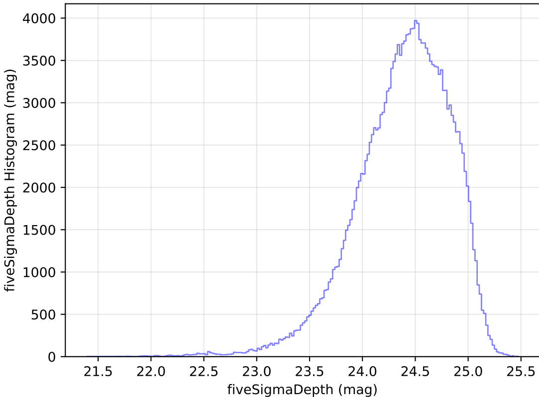
roll_pause_mjdp0_v3.4_10yrs g: fiveSigmaDepth Histogram
