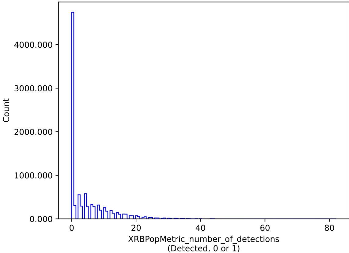
roll_pause_mjdp0_v3.4_10yrs : XRBPoMetric_number_of_detections
