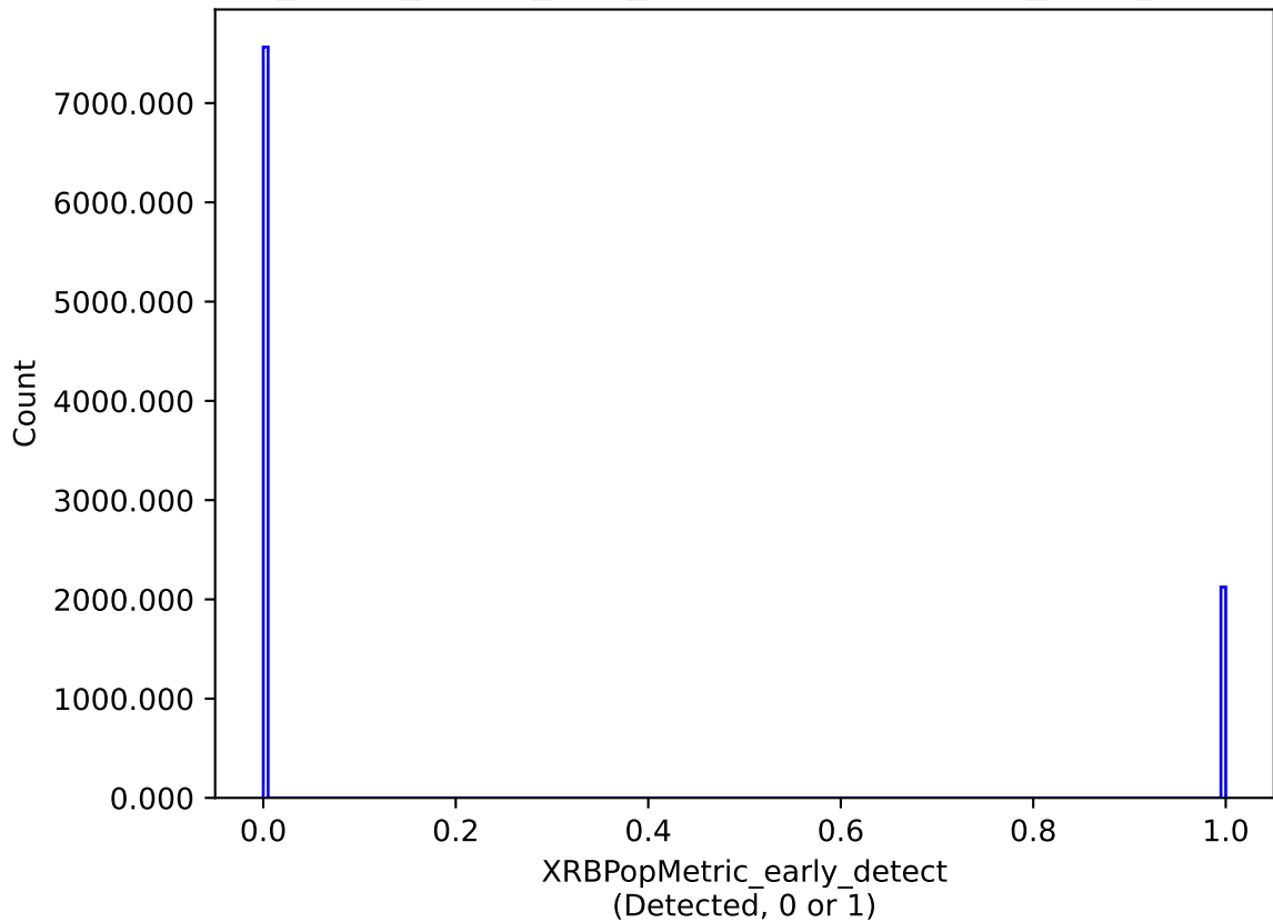
roll_pause_mjdp0_v3.4_10yrs : XRBPoMetric_early_detect
