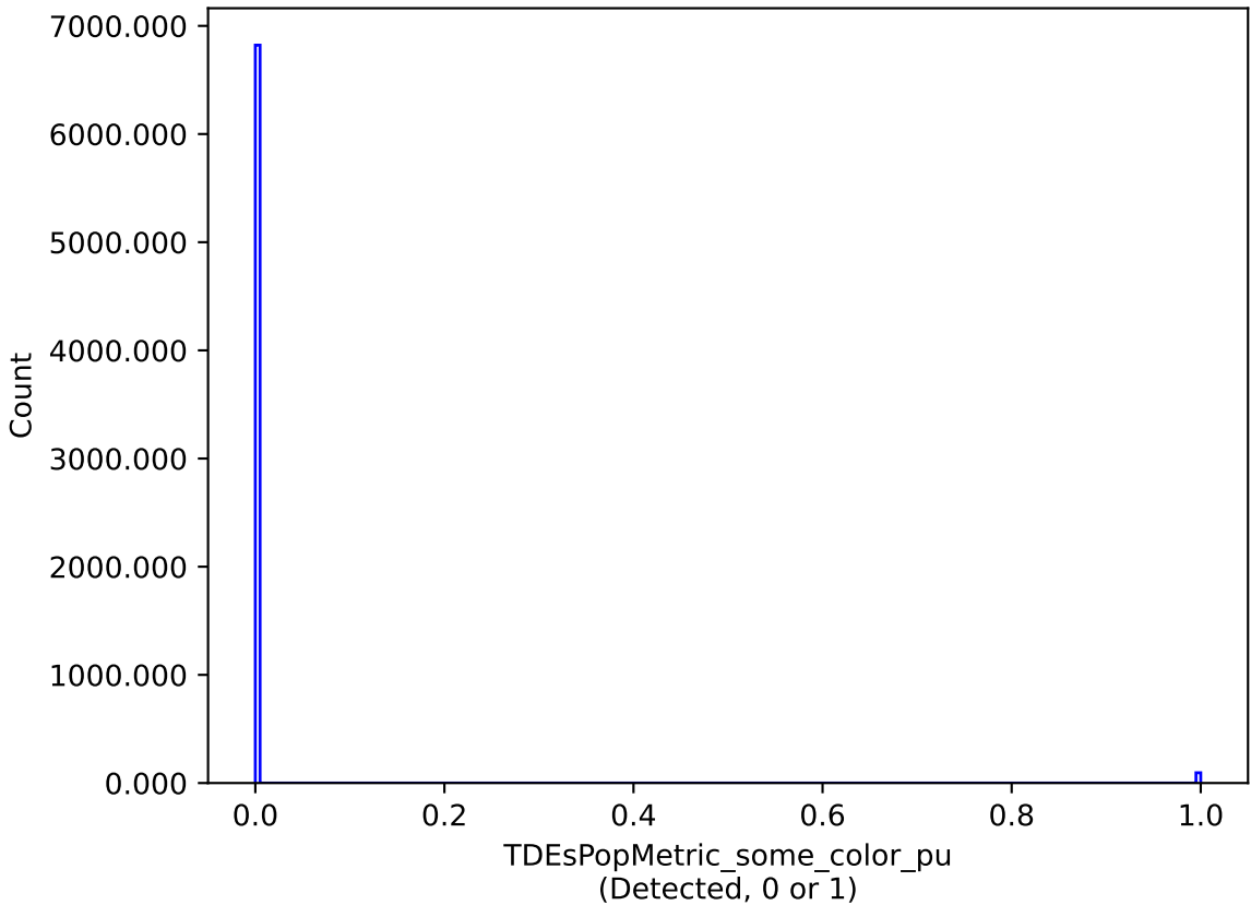
roll_pause_mjdp0_v3.4_10yrs : TDEsPopMetric_some_color_pu
