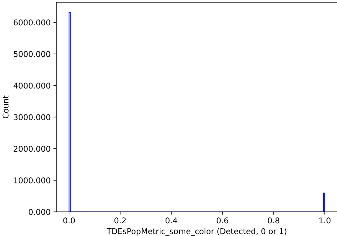
roll_pause_mjdp0_v3.4_10yrs : TDEsPopMetric_some_color
