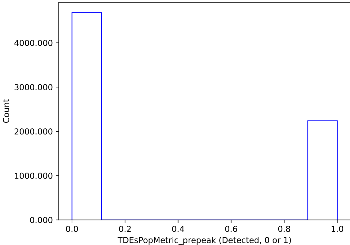
roll_pause_mjdp0_v3.4_10yrs : TDEsPopMetric_prepeak
