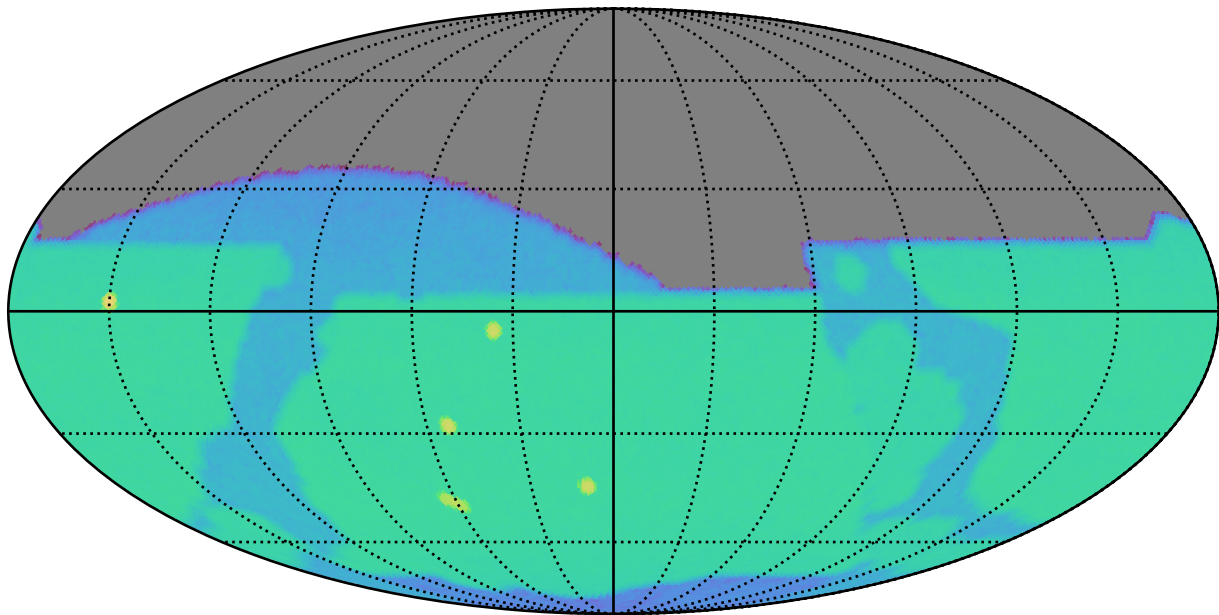
roll_pause_mjdp0_v3.4_10yrs z: SurfaceBrightLimit
