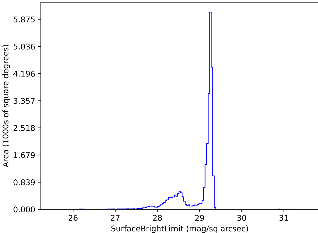
roll_pause_mjdp0_v3.4_10yrs z: SurfaceBrightLimit
