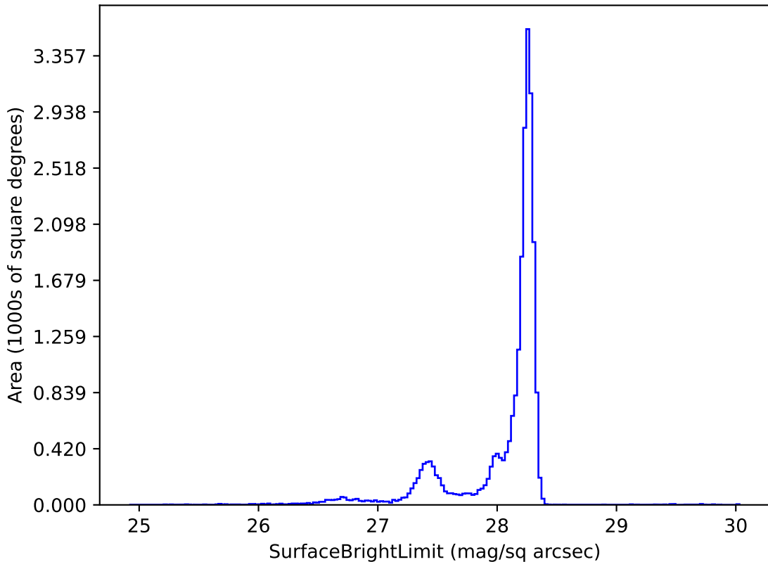
roll_pause_mjdp0_v3.4_10yrs y: SurfaceBrightLimit
