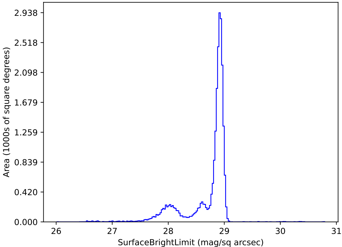
roll_pause_mjdp0_v3.4_10yrs u: SurfaceBrightLimit
