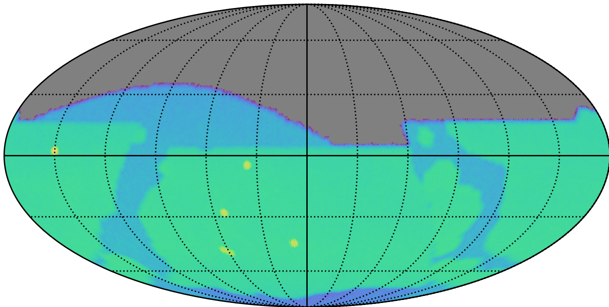
roll_pause_mjdp0_v3.4_10yrs r: SurfaceBrightLimit
