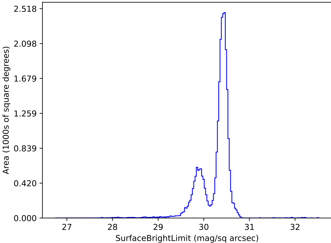
roll_pause_mjdp0_v3.4_10yrs g: SurfaceBrightLimit
