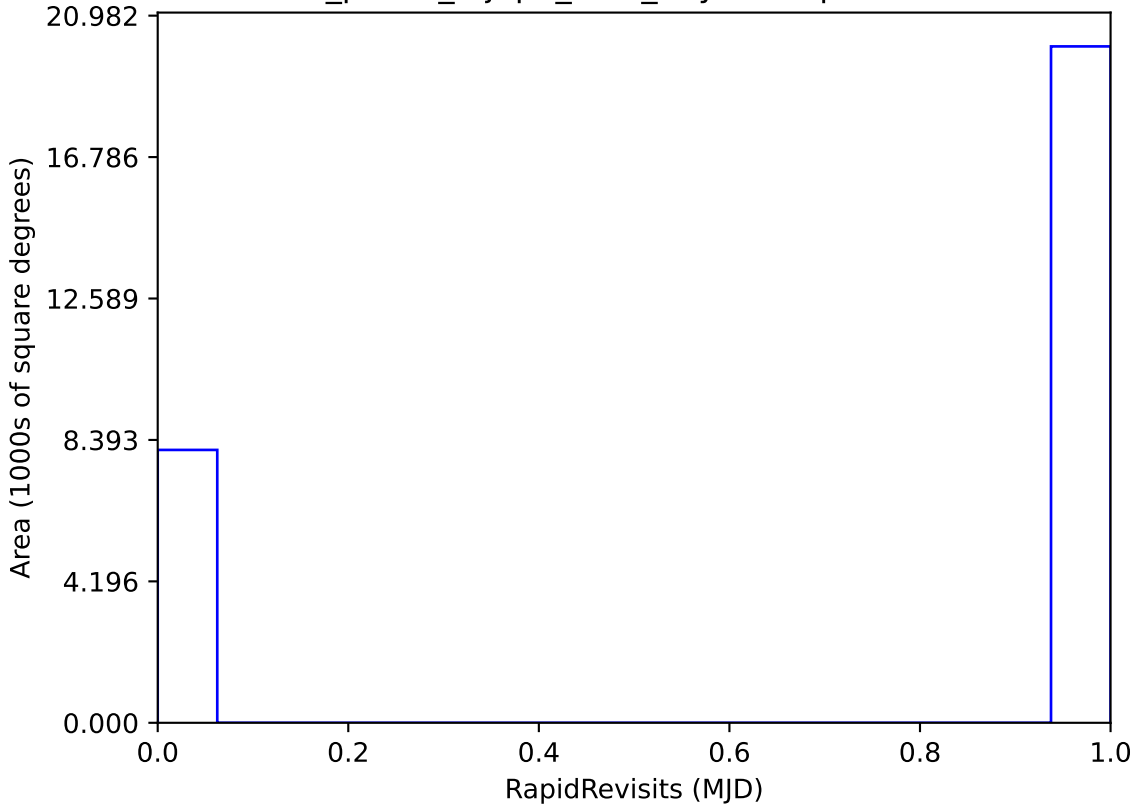
roll_pause_mjdp0_v3.4_10yrs : RapidRevisits
