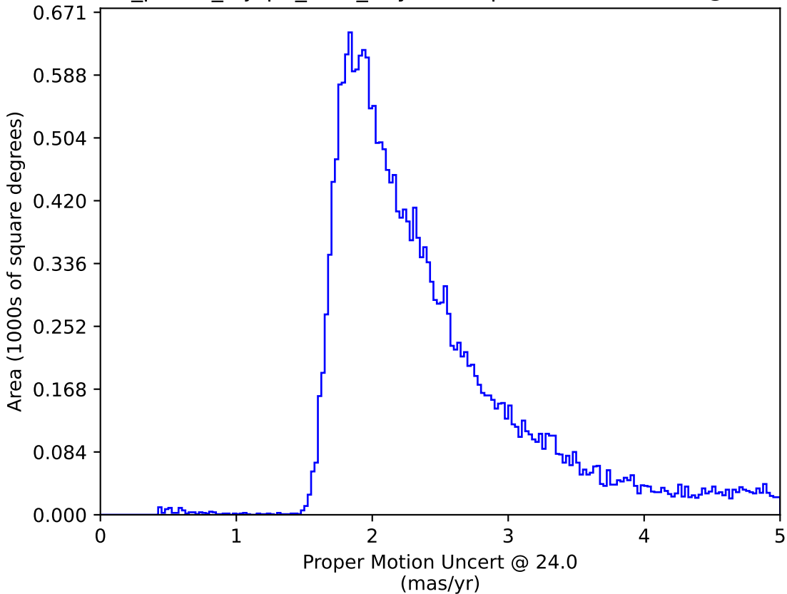
roll_pause_mjdp0_v3.4_10yrs : Proper Motion Uncert @ 24.0
