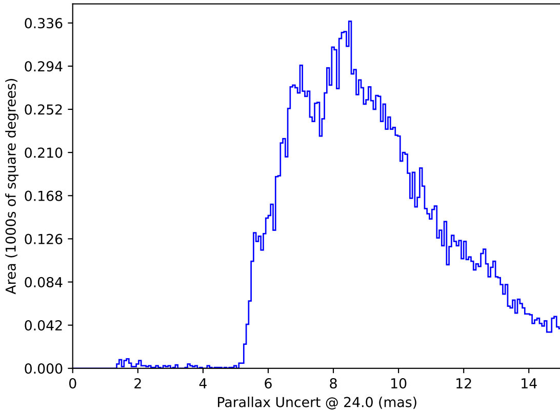
roll_pause_mjdp0_v3.4_10yrs : Parallax Uncert @ 24.0
