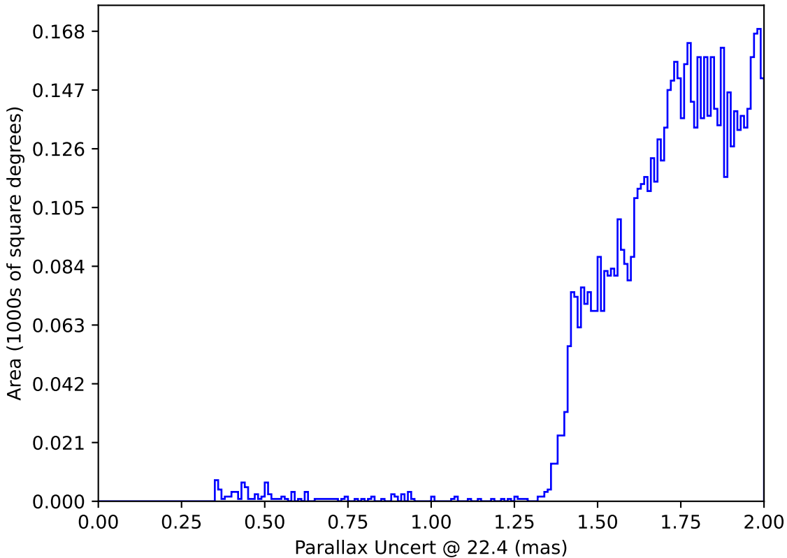
roll_pause_mjdp0_v3.4_10yrs : Parallax Uncert @ 22.4
