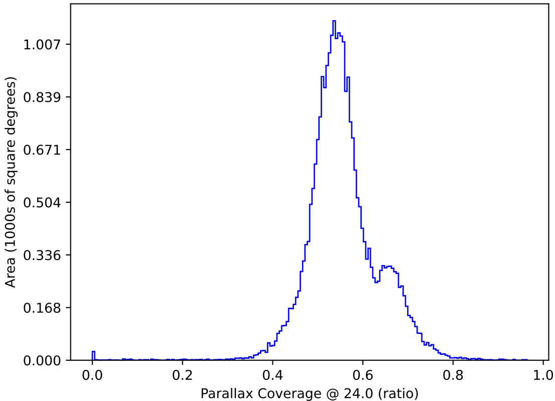
roll_pause_mjdp0_v3.4_10yrs : Parallax Coverage @ 24.0
