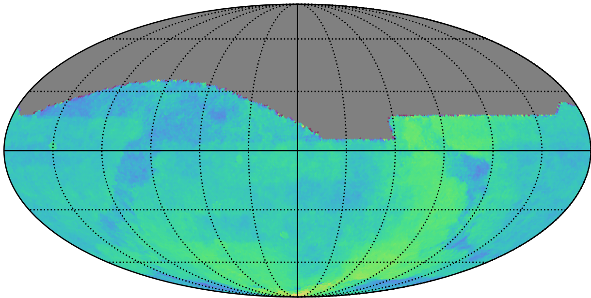
roll_pause_mjdp0_v3.4_10yrs : Parallax Coverage @ 22.4
