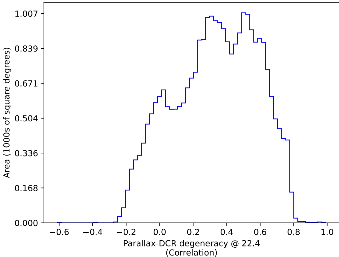
roll_pause_mjdp0_v3.4_10yrs : Parallax-DCR degeneracy @ 22.4
