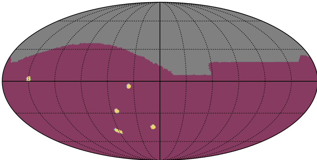
roll_pause_mjdp0_v3.4_10yrs : NumberOfQuickRevisits
