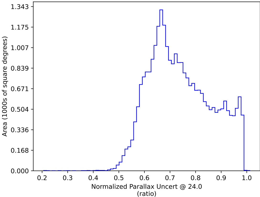
roll_pause_mjdp0_v3.4_10yrs : Normalized Parallax Uncert @ 24.0
