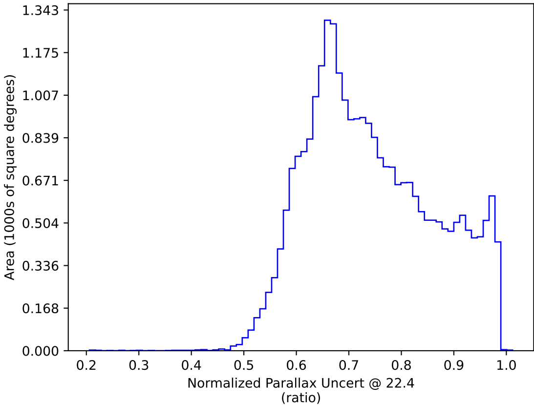
roll_pause_mjdp0_v3.4_10yrs : Normalized Parallax Uncert @ 22.4
