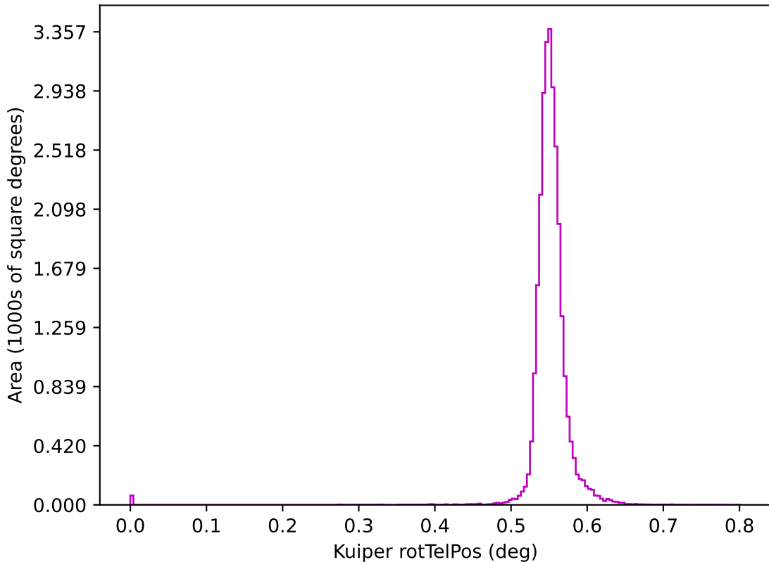
roll_pause_mjdp0_v3.4_10yrs z: Kuiper rotTelPos
