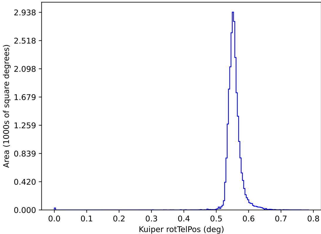
roll_pause_mjdp0_v3.4_10yrs y: Kuiper rotTelPos
