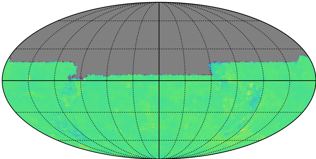
roll_pause_mjdp0_v3.4_10yrs u: Kuiper rotTelPos
