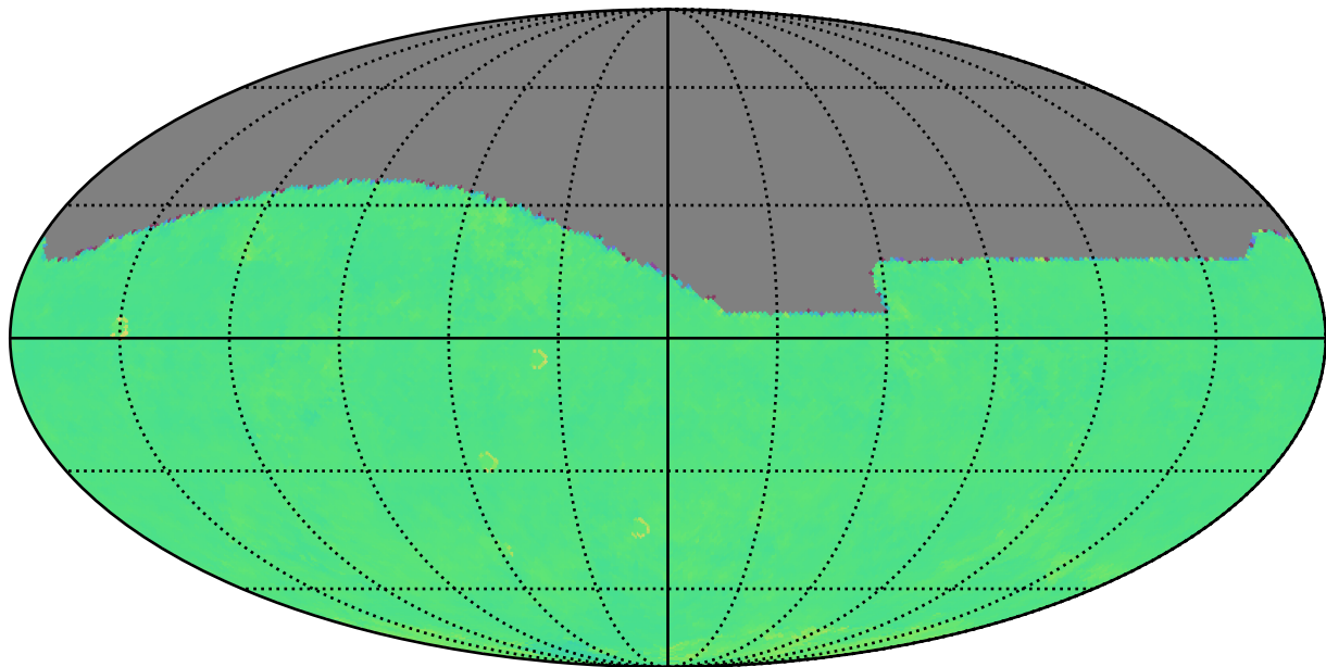
roll_pause_mjdp0_v3.4_10yrs r: Kuiper rotTelPos
