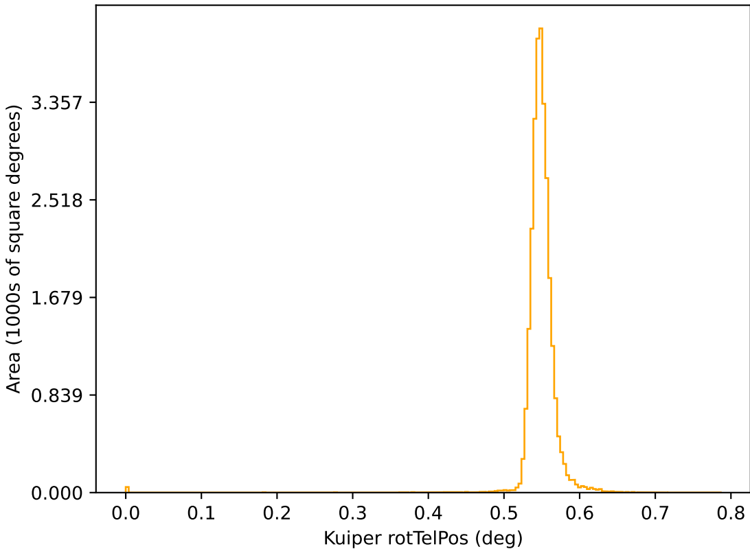
roll_pause_mjdp0_v3.4_10yrs r: Kuiper rotTelPos
