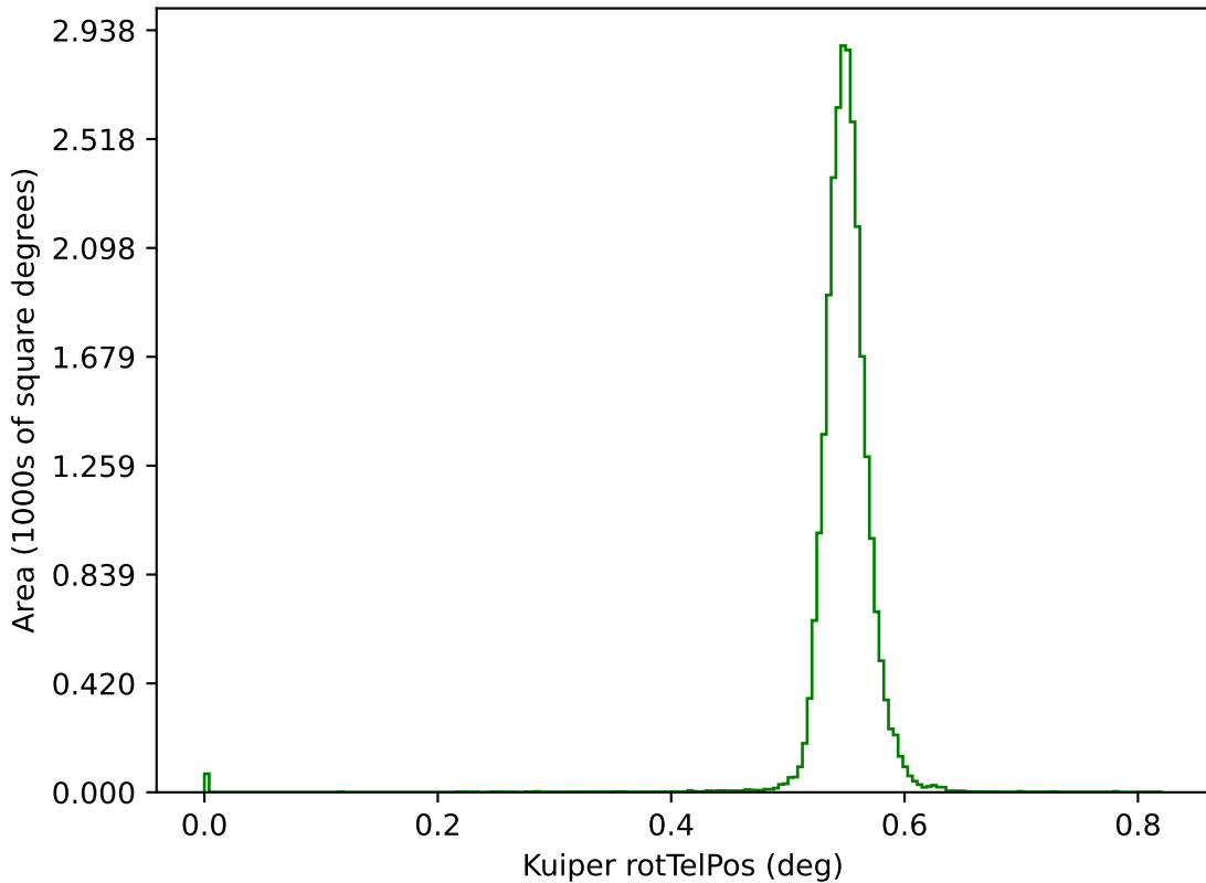
roll_pause_mjdp0_v3.4_10yrs g: Kuiper rotTelPos
