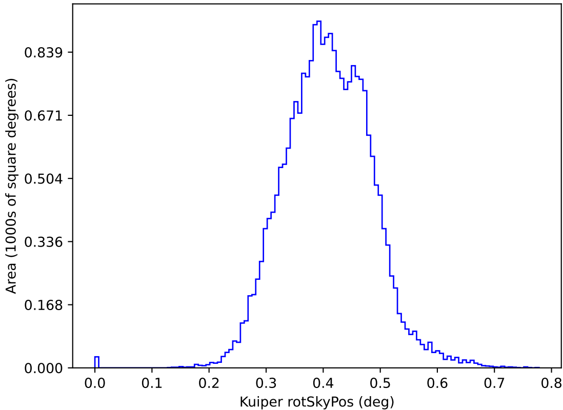
roll_pause_mjdp0_v3.4_10yrs y: Kuiper rotSkyPos
