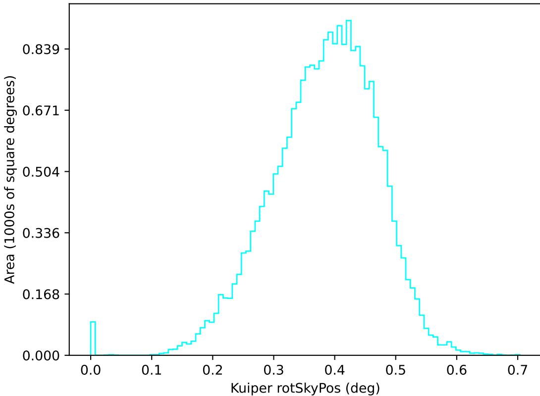
roll_pause_mjdp0_v3.4_10yrs u: Kuiper rotSkyPos
