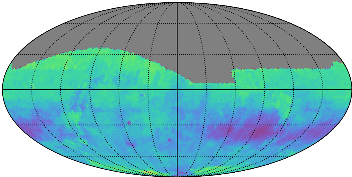
roll_pause_mjdp0_v3.4_10yrs r: Kuiper rotSkyPos
