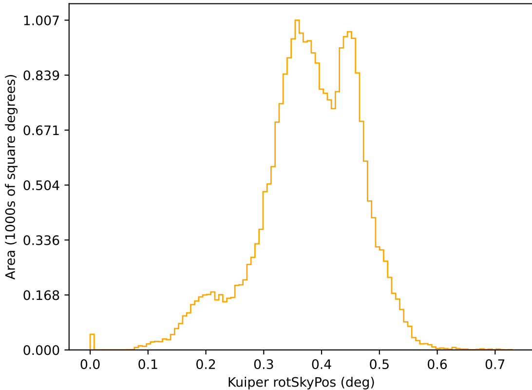
roll_pause_mjdp0_v3.4_10yrs r: Kuiper rotSkyPos
